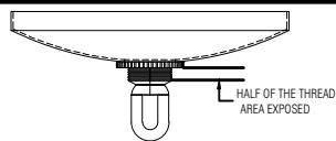
Drawing 2 – Canopy Adjustment
