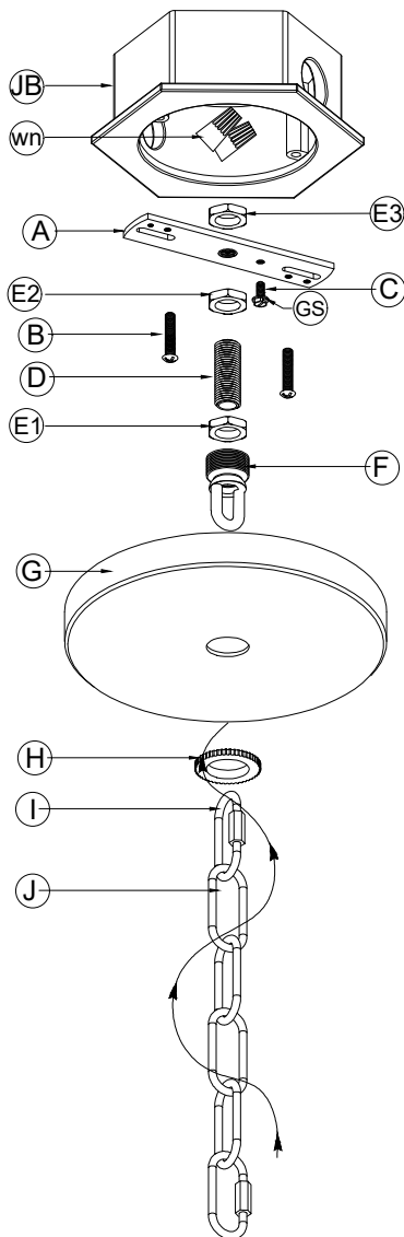
Drawing 1 – Hanging Instruction
